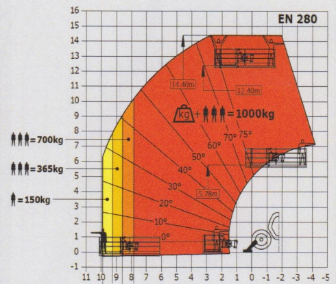
Machine on stabilizers with platform
