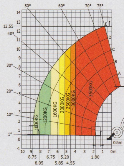
Machine on stabilizers with forks
